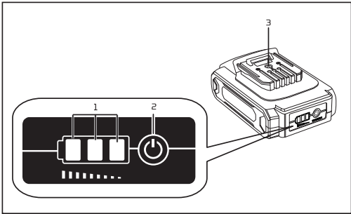
1. Indicator lamps 2. Check button, 3.DC port
