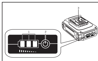
1. Indicator lamps 2. Check button. 3. DC port
