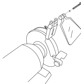
Installing Eye Shield to Grinder
