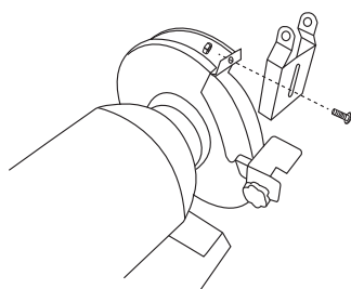
Installing Spark Guards
